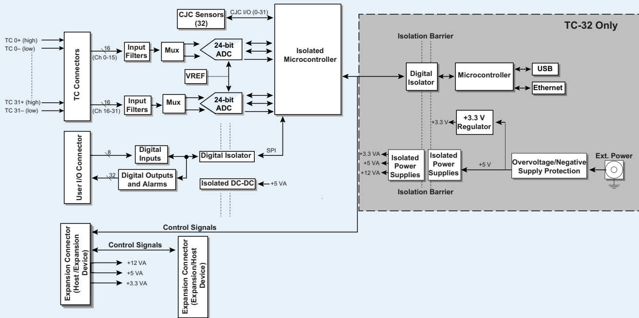
TC-32 and TC-32-EXP Block Diagram
